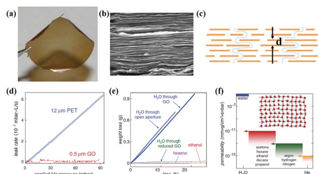
Fig. 5 (a) Photograph of a 1 μm-thick GO film; (b) SEM of the film's cross-section; (c) schematic view for possible permeation; (d) He-leak measurements for a GO membrane and a reference PET film; (e) weight loss for a container sealed with a GO film; (f) permeability of GO with respect to water and various small molecules. 52,53
