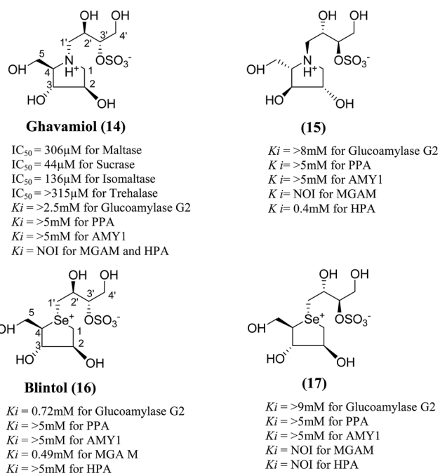
Fig. 7 Nitrogen ( 14 and 15 ) and selenium ( 16 and 17 ) heteroatom analogues of salacinal and their inhibition potential against \alpha -glucosidase enzymes.
