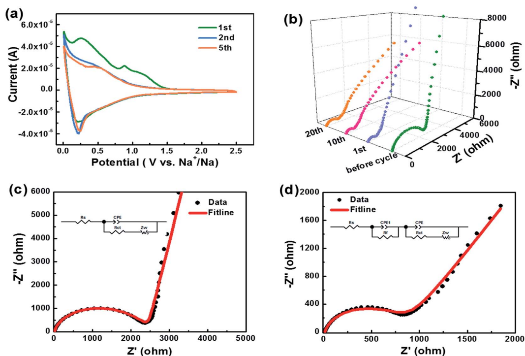
Fig. 6 (a) Cyclic voltammogram curves of sample HC-1000 at a scan rate of 0.1 mV s -1 between 0.01 and 2.5 V. (b) Nyquist plot deduced from EIS measurements of as prepared cells before cycle, after 1st, 10th and 20th cycle. (c) The fitline of Nyquist plot and equivalent circuit used to fit the EIS of sample HC-1000 before cycle and (d) after 20th cycle.
