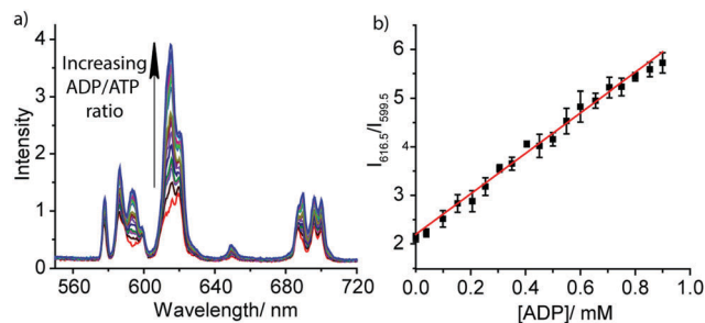
Fig. 3 (a) Ratiometric change in emission spectra of [\text{Eu.1}]^+ ( 8 \mu\text{M} ) in the presence of increasing ratio of ADP/ATP; (b) plot of the emission intensity ratio, 616.5/599.5 \text{ nm} , versus mole fraction of ADP. Conditions: buffered aqueous solution ( 10 \text{ mM} HEPES, \text{pH } 7.0 ) containing \text{MgCl}_2 ( 3 \text{ mM} ). Concentration of ADP: 0\text{--}0.9 \text{ mM} , total nucleoside concentration = 1 \text{ mM} . \lambda_{\text{exc}} = 330 \text{ nm} , 298 \text{ K} .
