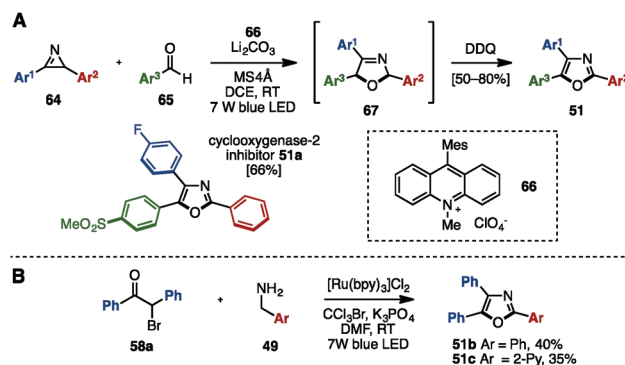
Scheme 13 Triarylloxazole synthesis enabled by photoredox catalysis.
