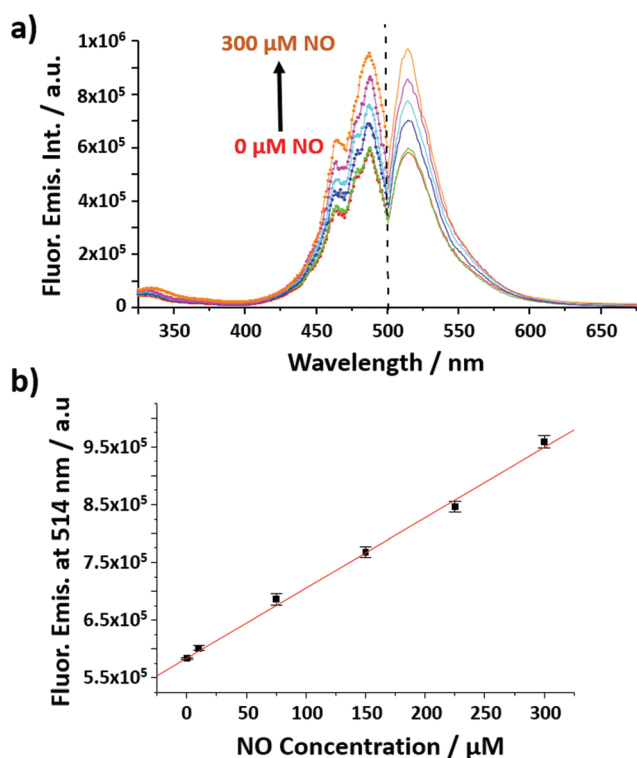
Fig. 2 (a) Fluorescence excitation (left; \lambda_{\text{exc}} = 514 \text{ nm} ) and emission (right; \lambda_{\text{exc}} = 492 \text{ nm} ) spectra of the NO nanobiosensor in the presence of increasing concentrations of NO (from 0 to 300 \mu\text{M} ). (b) Calibration curve of the NO nanobiosensor obtained from the fluorescence emission intensity at 514 nm as a function of the concentrations of NO; error bars show the mean error of 3 replicates. y = 1217x + 584141 .
