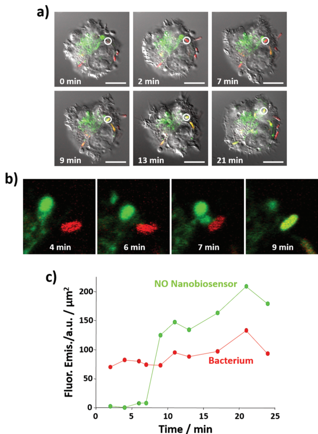
Fig. 7 Time course of NO generation during bacterial phagocytosis as measured by the NO nanobiosensor. (a) Confocal fluorescence microscopy images of live RAW264.7 \text{NO}^- cells stimulated with IFN- \gamma ( 10 \text{ ng mL}^{-1} ) and LPS ( 500 \text{ ng mL}^{-1} ) and incubated with the NO nanobiosensor ( 10 \text{ nM} ) overnight, and then challenged with Texas Red stained E. coli bacteria for 3 h prior to imaging. The images, taken at t = 0, 2, 7, 9, 13 and 21 \text{ min} , are composite images of the green (NO nanobiosensor, \lambda_{\text{exc}} = 488 \text{ nm} , emission collected between 505 and 545 \text{ nm} ), red (Texas Red tagged E. coli , \lambda_{\text{exc}} = 543 \text{ nm} , emission collected between 560 and 750 \text{ nm} ) and DIC channels ( \lambda_{\text{exc}} = 488 \text{ nm} ). Images were captured using the 'line by line' function of a Zeiss LSM 510 confocal microscope. The white circle indicates a region of interest where an E. coli fragment co-localises with the NO nanobiosensor at t = 9 \text{ min} . Scale bars = 10 \mu\text{m} . (b) Magnified image of the region where the NO nanobiosensor co-localises with the E. coli fragment in (a) at t = 4, 6, 7 and 9 \text{ min} . (c) Fluorescence emission intensity, plotted as the mean value per unit area, of the NO nanobiosensor (green) and the Texas Red tagged E. coli (red) as a function of time.
