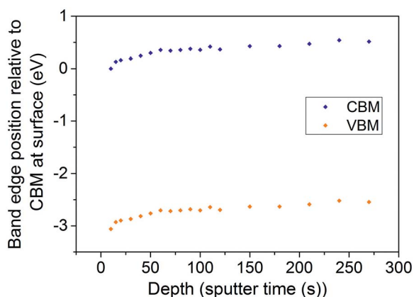
Fig. 7 VBM and CBM variation with depth in a Sb/Rh codoped \text{TiO}_2 (110) crystal. The CBM at the surface is placed at 0 eV and the band gap is assumed to be 3.06 eV as in bulk rutile \text{TiO}_2 . The Sb/Rh dopant ratio was measured by XPS depth profiling. This was correlated with the Fermi level shifts as described in the text.
