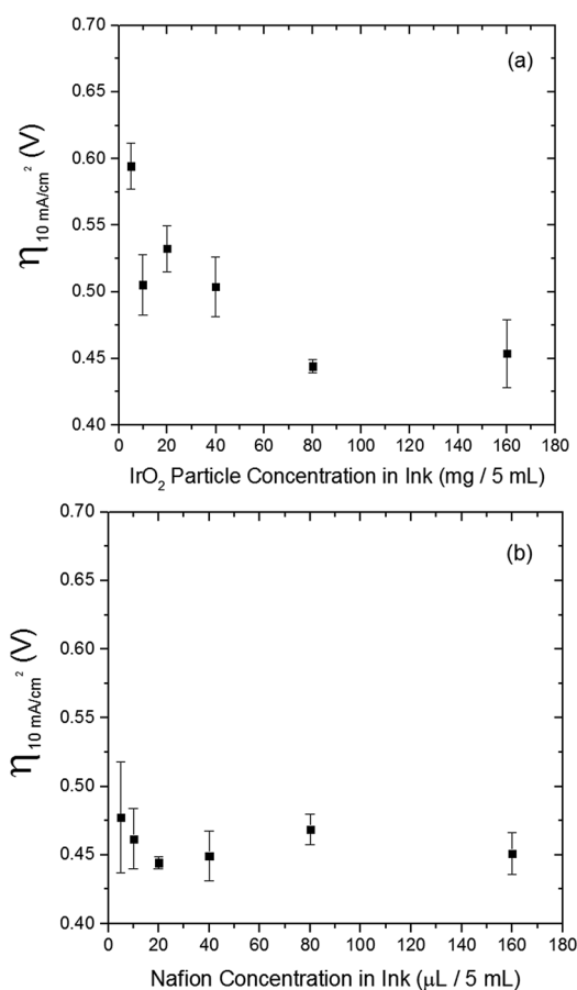
Fig. 2 The effects of IrO₂-(i) particle and Nafion concentrations for the drop-cast on overpotential values at 10 \text{mA cm}_{\text{geo}}^{-2} in 1 M NaOH. (a) Effect of IrO₂-(i) particle concentration on OER overpotential at a fixed Nafion concentration of 40 \mu\text{L} in 5 mL solution. The overpotential value decreases as the iridium oxide loading increases, and then plateaus at around 80 \text{mg}/5 \text{ mL} . (b) Effect of Nafion concentration on OER overpotential at a fixed IrO₂-(i) loading of 80 \text{mg} in 5 mL solution. The Nafion concentration does not appear to influence the overpotential values significantly, but the overpotential shows relatively high variations in very small concentration ranges (5–10 \mu\text{L}/5 \text{ mL} ), which can be attributed to catalyst adherence issues. The overpotential measurements were conducted with RDEV at 1600 rpm and a scan rate of 10 \text{mV s}^{-1} .
