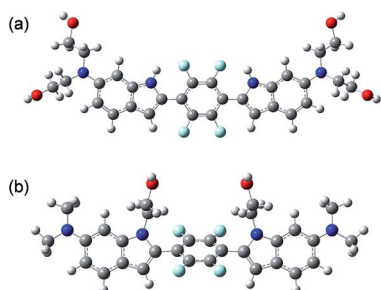
Fig. 2 DFT optimized geometries of the cis -isomer of (a) QAD1 and (b) 3 in EtOH.
