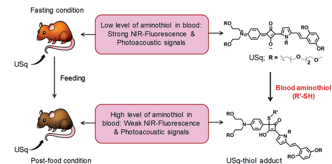
Scheme 1 Schematic diagram depicting the realization of fluorescence and photoacoustic bimodal signaling of aminothiols content in vivo using USq.
