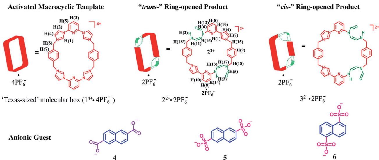
Scheme 1 Structures of the "Texas-sized" molecular box ( 1 4+ ·4PF 6 − ) and its "trans-" and "cis-" imidazolium ring-opened products. Also shown are the dianionic guest molecules used in this study.
