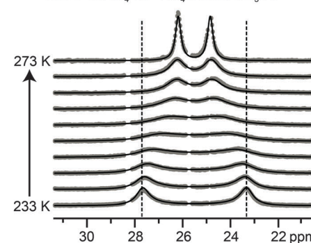
Fig. 5 Detection of screw-sense preference by NMR in the fast exchange regime. (a and b) Coalescence between signals in an equally populated pair of enantiomeric conformers; (c and d) coalescence between signals in an unequally populated pair of diastereoisomeric conformers.
