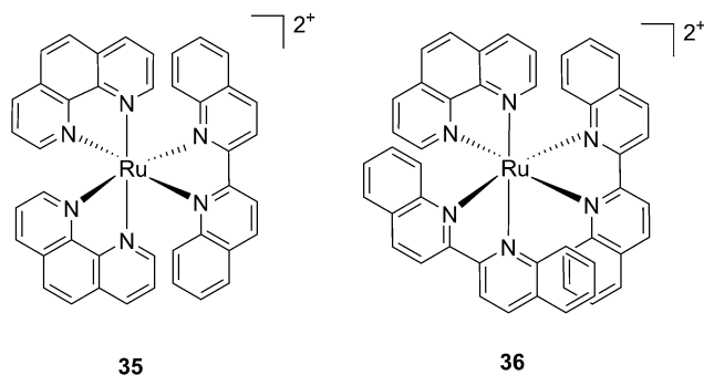
Fig. 27 Structures of the two Ru(II) complexes 35 and 36 with the biq ligands that are exchanged upon irradiation. 86
