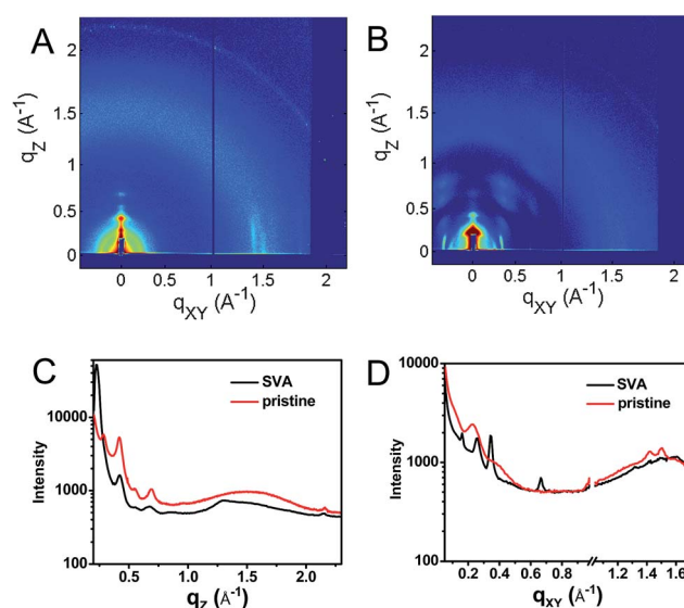
Fig. 3 GIWAXS of a pristine (A) film of 1 and a film which has been solvent vapor annealed in \text{CH}_2\text{Cl}_2 for 10 min (B) as well as vertical (C, q_{xy} = 0 ) and horizontal (D, q_z = 0 ) line cuts of the annealed (black) and unannealed (red) films.
