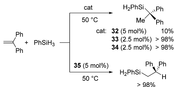
Scheme 9 Hydrosilylation of diphenylethylene catalysed by 32–35 .
