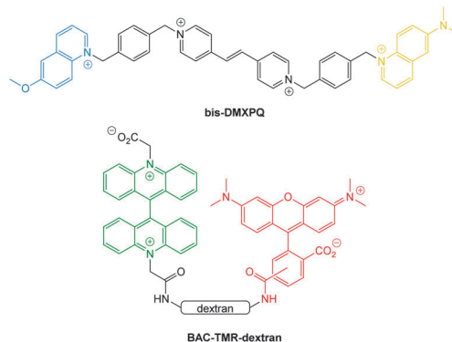
Fig. 20 Ratiometric probes bis-DMXPQ and BAC-TMR-dextran used for chloride imaging.
