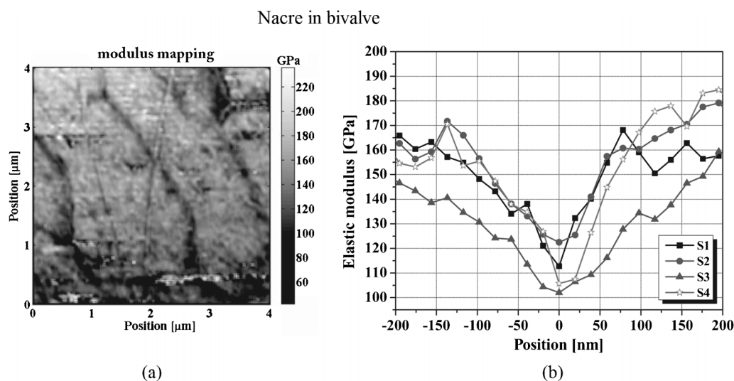
Fig. 18 (a) Map of elastic modulus taken from the nacre layer at a depth of 300 \mu\text{m} beneath the inner surface of the bivalve shells of Perna canaliculus ; (b) the modulus change across organic-inorganic interfaces. 110
