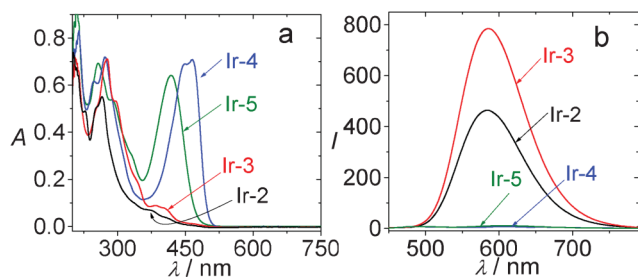
Fig. 19 (a) UV-vis absorption of Ir-2 , Ir-3 , Ir-4 and Ir-5 . In \text{CH}_3\text{CN} ( 1.0 \times 10^{-5} \text{ M} ; 20^\circ \text{C} ). (b) Emission spectra of the \text{Ir}^{\text{III}} complexes. Ir-2 : \lambda_{\text{ex}} = 386 \text{ nm} , Ir-3 : \lambda_{\text{ex}} = 407 \text{ nm} , Ir-4 : \lambda_{\text{ex}} = 462 \text{ nm} , Ir-5 : \lambda_{\text{ex}} = 421 \text{ nm} . In deaerated \text{CH}_3\text{CN} ( 1.0 \times 10^{-5} \text{ M} ; 20^\circ \text{C} ). Reproduced with permission from ref. 45b.
