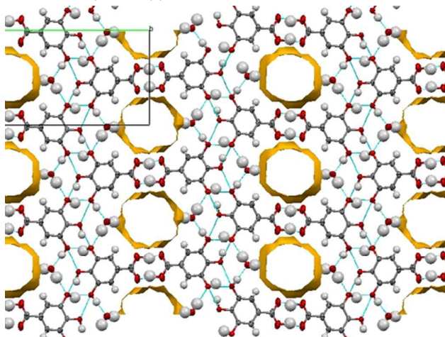
Figure 4. Channels observed in the porous form of gallic acid monohydrate (4-H 2 O).
