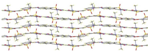
Figure 3. Layers in the piroxicam: methanol (3:1) solvate, 1-MeOH .
