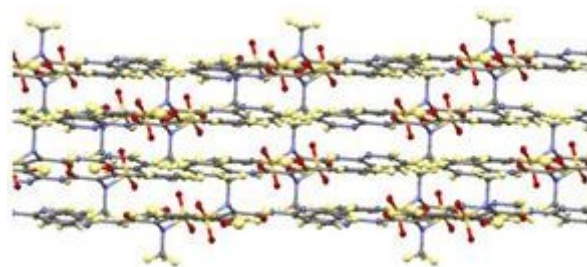
Figure 2. The layered arrangement of molecule in the crystal packing in piroxicam form III, 1-III .
