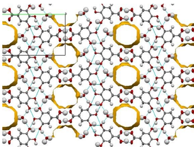
Figure 4. Channels observed in the porous form of gallic acid monohydrate (4-H 2 O).
