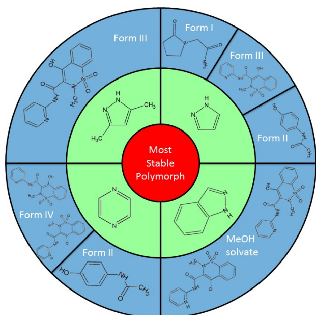
Figure 1: Multi-component routes to elusive polymorphs of piroxicam, piracetam and paracetamol. In this schematic, the green ring represents the various N-heterocycles employed, the outer blue ring the target molecules, detailing the forms produced by the templating approach.
