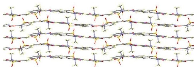
Figure 3. Layers in the piroxicam: methanol (3:1) solvate, 1-MeOH .
