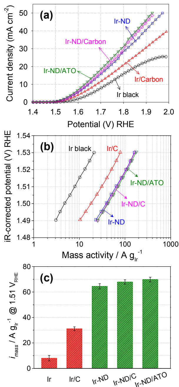
Figure 5. The electrocatalytic OER activities of Ir-ND, Ir-ND/C and Ir-ND/ATO. For comparison, commercial Ir black and synthesized Ir/C by polyol process were also evaluated under same condition. (a) The polarization curve for OER of electrocatalysts in three electrode system, (b) iR-corrected Tafel plots from the polarization curve, (c) Ir-mass based activity at \eta = 280 \text{ mV} overpotential (1.51 V RHE ). All the measurements were performed in \text{N}_2 -purged 0.05 M \text{H}_2\text{SO}_4 . Catalysts loading: 10.2 \mu\text{g}_{\text{Ir}}\text{cm}^{-2} . Scan rate: 5 \text{ mVs}^{-1} .
