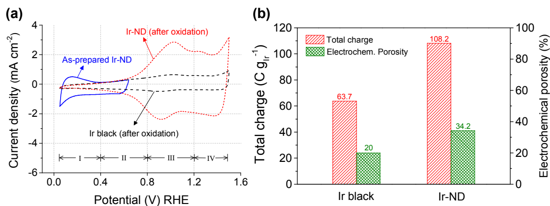
Figure 3. Surface redox electrochemistry of commercial Iridium black and Iridium Nanodendrites (Ir-ND): (a) Cyclic voltammograms (CVs) of as-prepared and oxidized Nanodendrites. Conditions: 25 C, N 2 -purged 0.05 M H 2 SO 4 , 20 mV s -1 . The CV of the as-prepared Ir nanodendrites (Ir-ND) was recorded between +0.05 to +0.64 V RHE to avoid Ir oxide formation. (b) Electrochemical total charge and porosity of Ir-ND and Ir black.
