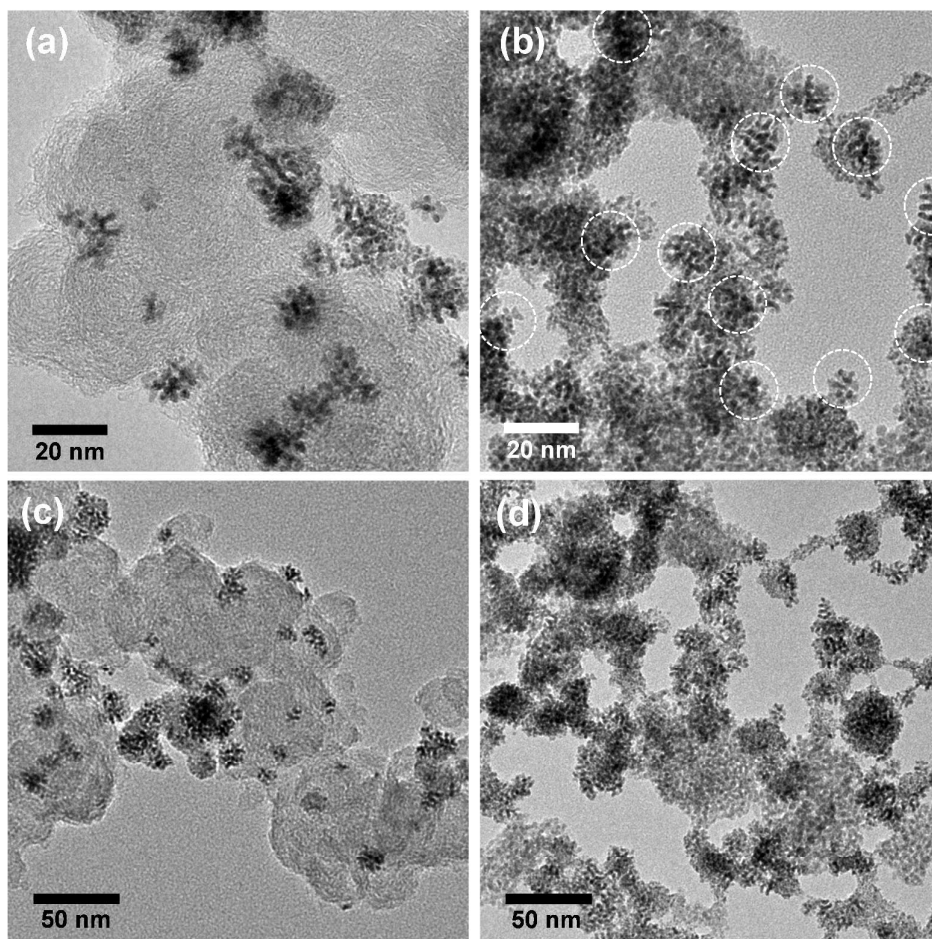
Figure 4. HR-TEM images of Ir-ND supported on (a) carbon black and (b) antimony-doped tin oxide (ATO). Low magnification TEM images of (c) Ir-ND/C and (d) Ir-ND/ATO.
