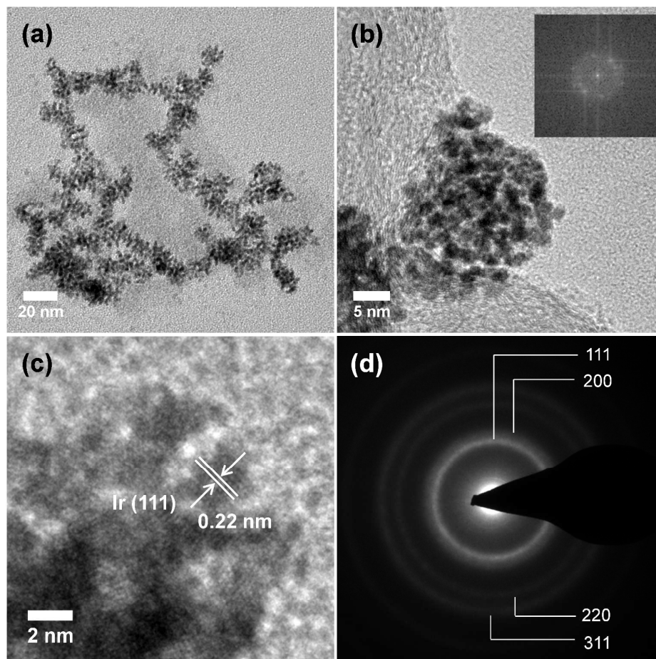
Figure 1. (a) Low and (b) high resolution TEM images of the Ir nanodendrites (Ir-ND) synthesized by reducing H_2IrCl_6 \cdot xH_2O with NaBH_4 in the presence of TTAB and the corresponding Fourier-transform (FT) pattern of the Ir-ND (inset b). (c) Magnified HRTEM image of one single Ir-ND and (d) the corresponding SAED pattern.
