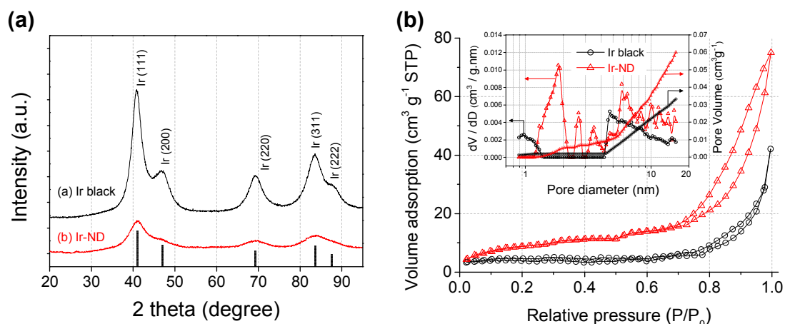
Figure 2. (a) XRD patterns of commercial Ir black and synthesized Ir-ND. (b) Nitrogen adsorption-desorption isotherms and pore size distribution (inset) of commercial Ir black and synthesized Ir-ND. Pore size distribution was calculated using non-local density functional theory (NLDFT).
