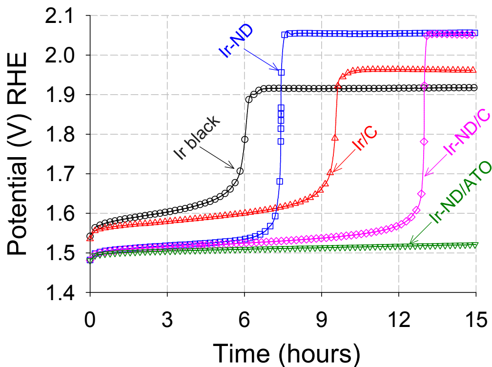
Figure 7. Accelerated constant current-load durability test (ADT) of Ir-ND OER electrocatalysts in comparison to reference catalysts measured under identical conditions. test time: 15 h, N_2 -purged condition, catalyst loading: 10.2 \mu g_{Ir} cm^{-2} , 1600 rpm, 10 mA cm^{-2} .
