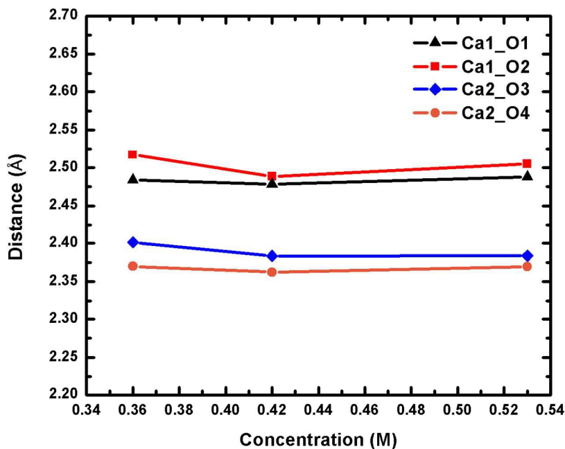
Fig. 4 Change of the four Ca-O eq distances of the Ca 2 UO 2 (CO 3 ) 3 complex in water at three different concentrations. See Fig. 1 for atom labels. The distances are averages over 15ps trajectories; the standard deviations for each datapoint are shown in Fig. S2 of the ESI.
