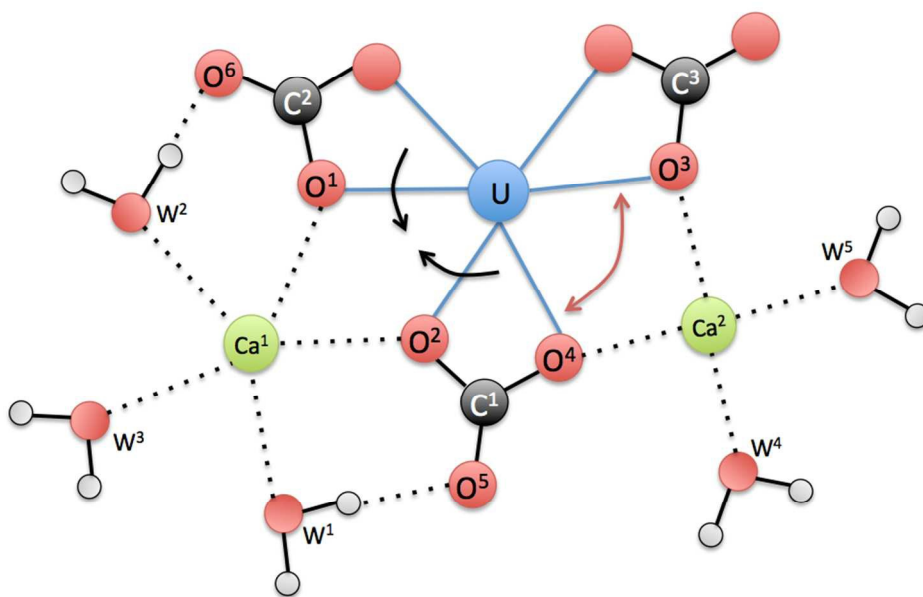
Figure 7. A schematic view of the equatorial plane around U for the \text{Ca}_2\text{UO}_2(\text{CO}_3)_3 complex in water. W stands for water.
