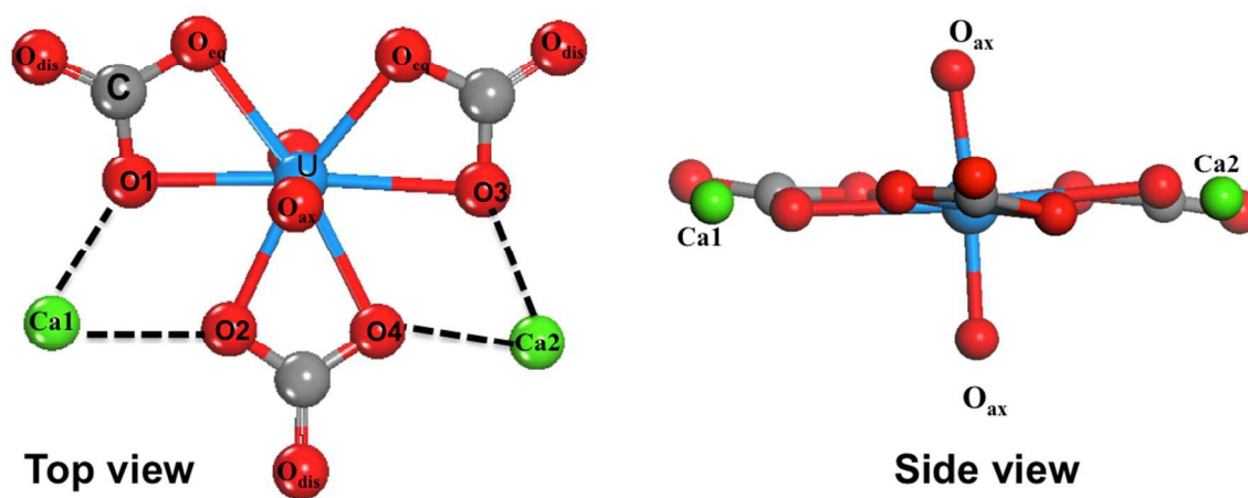
Fig. 1 Top view and side view of the Ca_2UO_2(CO_3)_3 complex in water.
