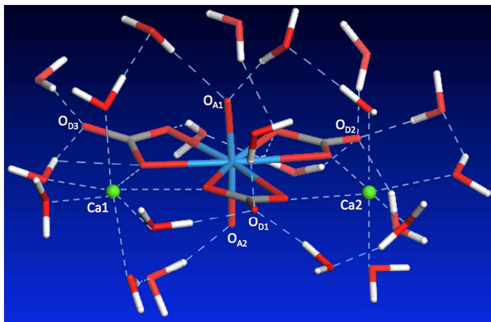
Figure 8. A snapshot of the first solvation shell of water molecules around the Ca 2 UO 2 (CO 3 ) 3 complex.
