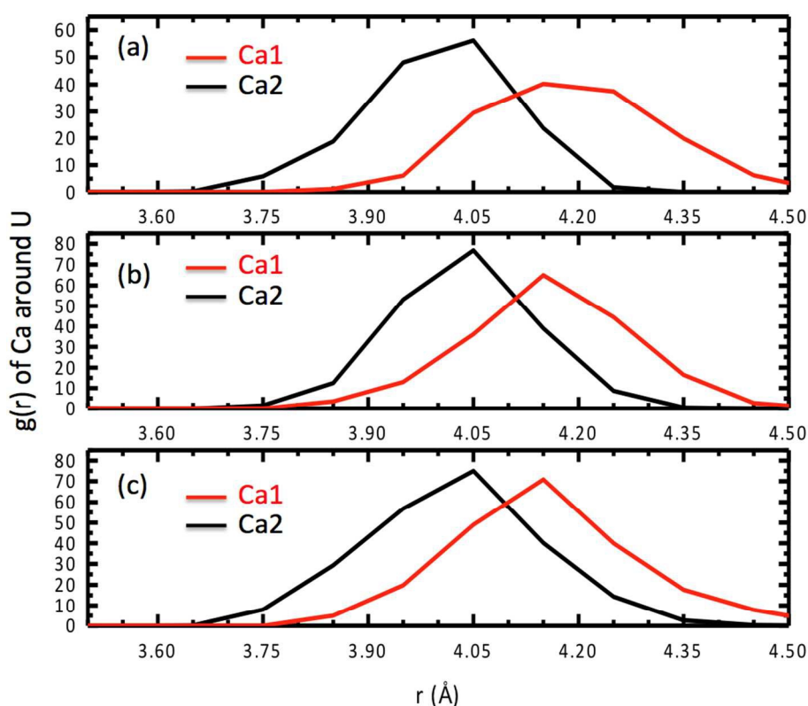
Fig. 9 Radial distribution functions of Ca ions around the U atom for three different concentrations of \text{Ca}_2\text{UO}_2(\text{CO}_3)_3 in water: (a) 0.53; (b) 0.43; (c) 0.36 M.
