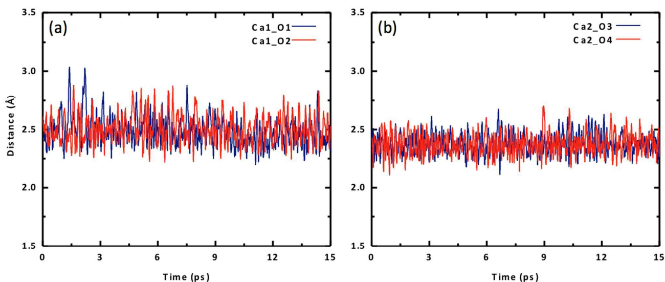
Fig. 2 Change of Ca-O distances with time for the \text{Ca}_2\text{UO}_2(\text{CO}_3)_3 complex in water (0.55 M): (a) Ca1-O1 and Ca1-O2; (b) Ca2-O3 and Ca2-O4. See Fig. 1 for atom labels.
