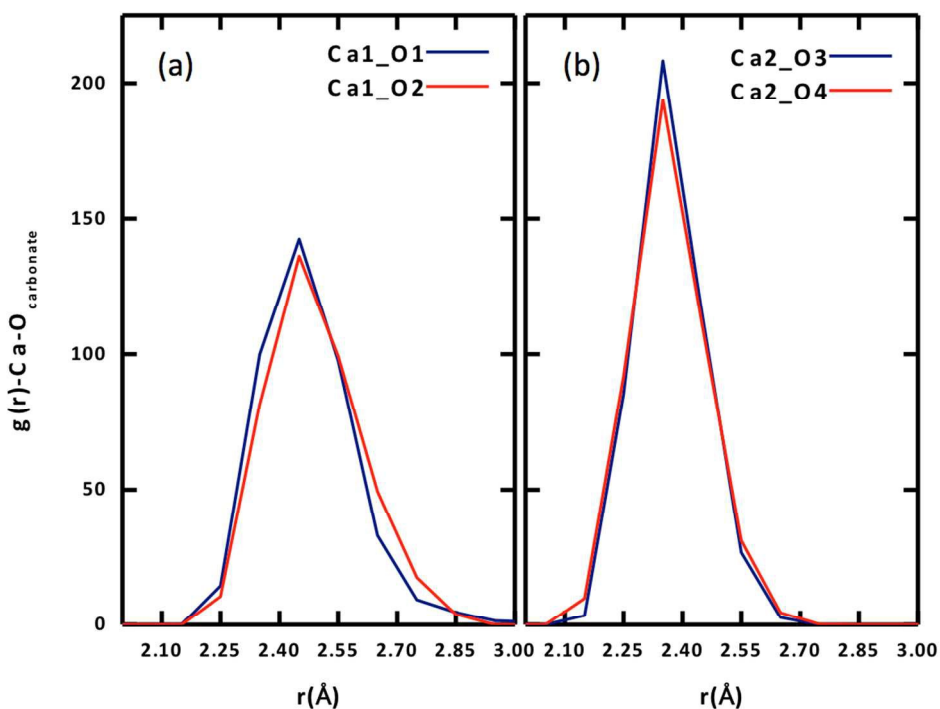
Fig. 3 Radial distribution functions of equatorial carbonate oxygen ( O_{\text{eq}} ) around each Ca ion of the \text{Ca}_2\text{UO}_2(\text{CO}_3)_3 complex in water (0.55 M): (a) Ca1; (b) Ca2. See Fig. 1 for atom labels.
