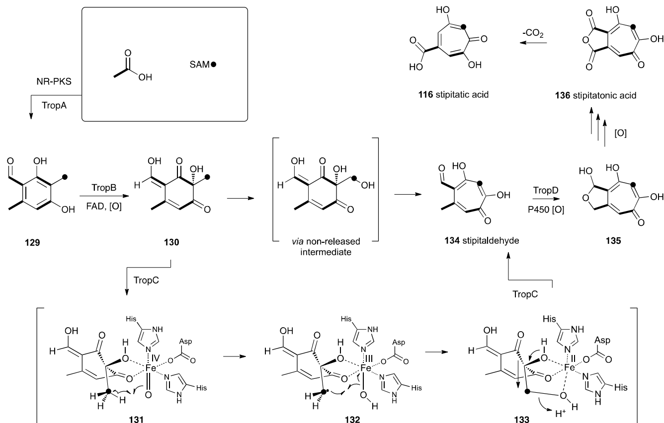
Scheme 21. Biosynthesis of tropolones.
