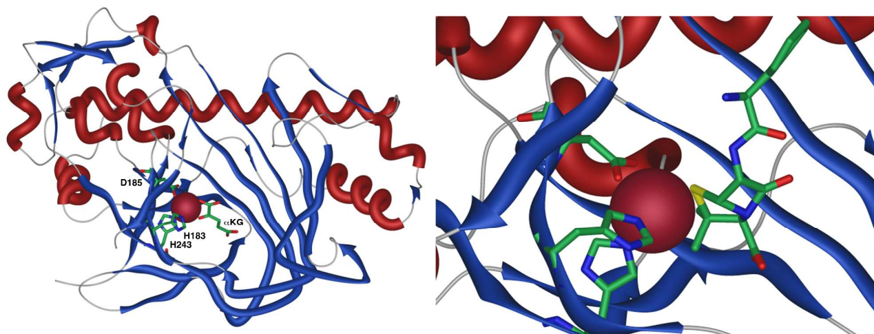
Figure 1. The overall structure of DAOCS showing the active site iron atom, key residues and substrates. Expansion shows ampicillin bound in active site. Coordinates from 1RXG and 1UNB respectively.
