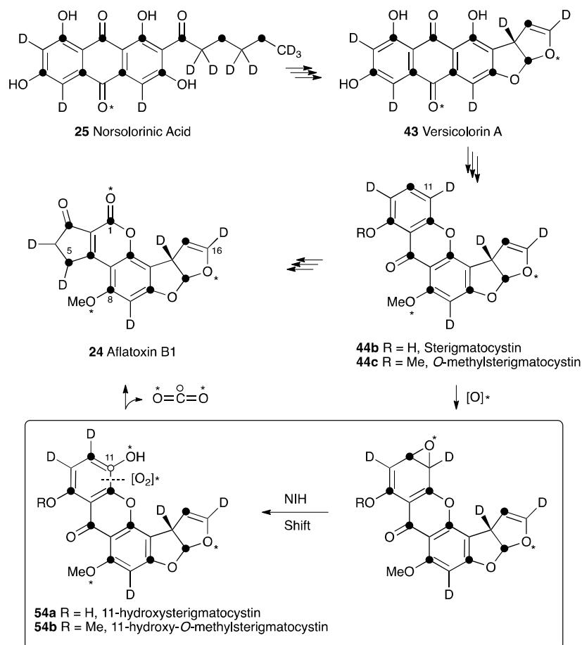
Scheme 11. Rationalisation of results obtained when feeding [2\text{-}^2\text{H}_3] acetate to A. parasiticus . Dark circles indicate positions of acetate C-1-derived carbons. Hollow circle shows fate of C-11. * = atmospheric oxygen.
