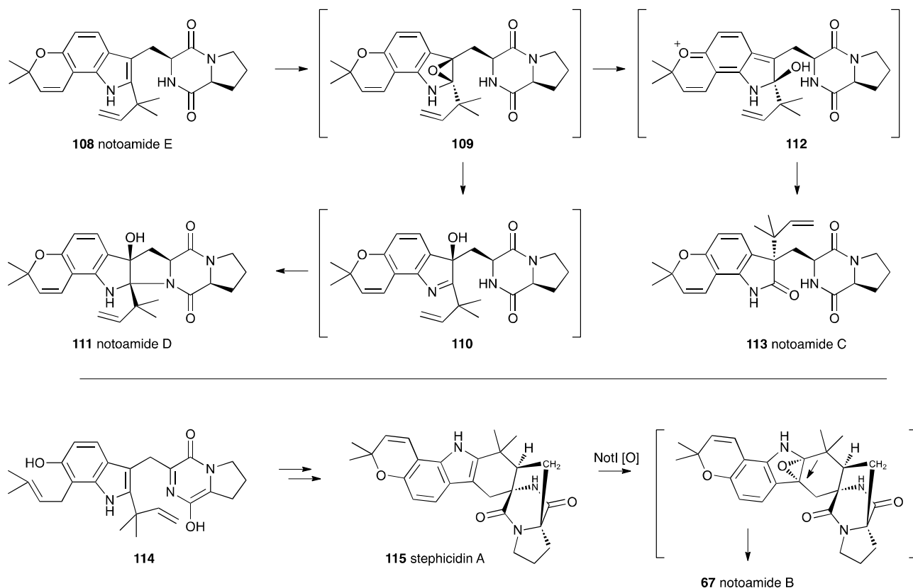
Scheme 19. Oxidative rearrangements involved in notoamide biosynthesis.
