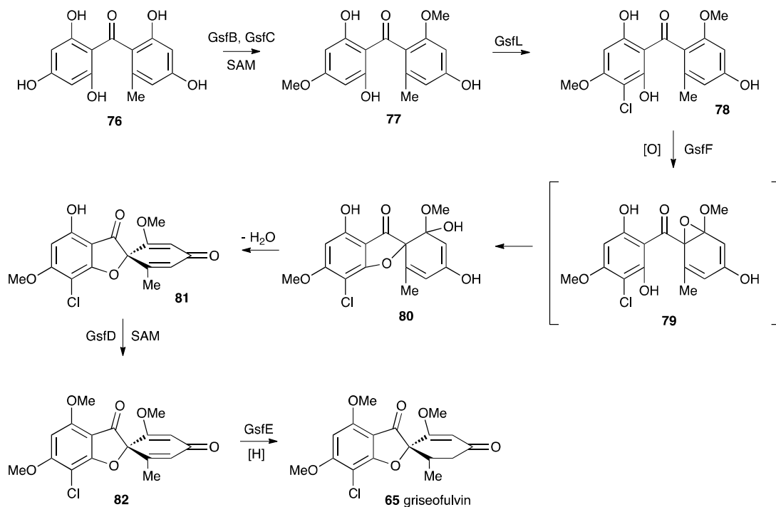
Scheme 14. Biosynthesis of griseofulvin 65 in Penicillium aethiopicum .
