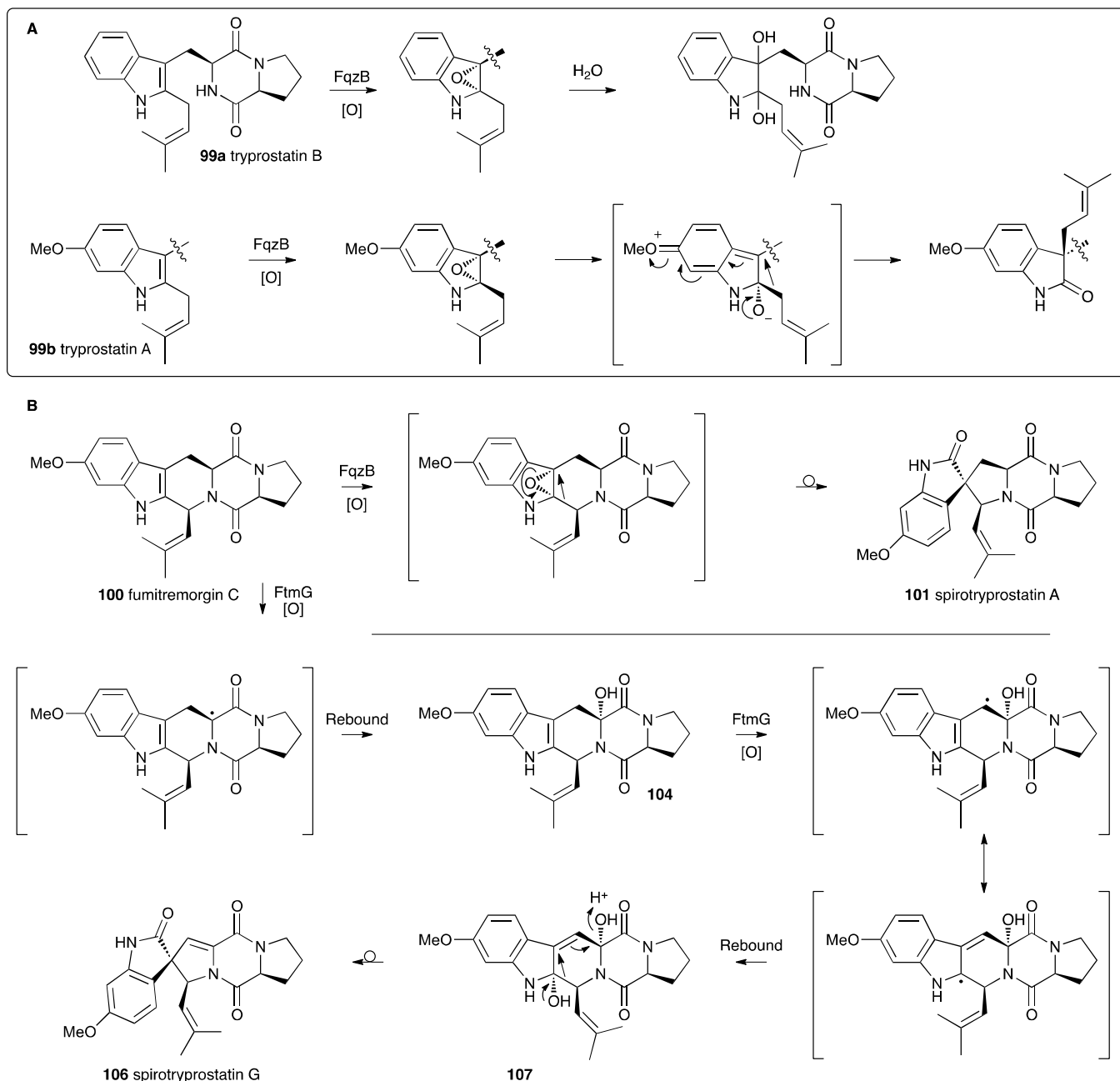
Scheme 18. Proposed oxidative rearrangement mechanisms during spirotryprostatin biosynthesis.
