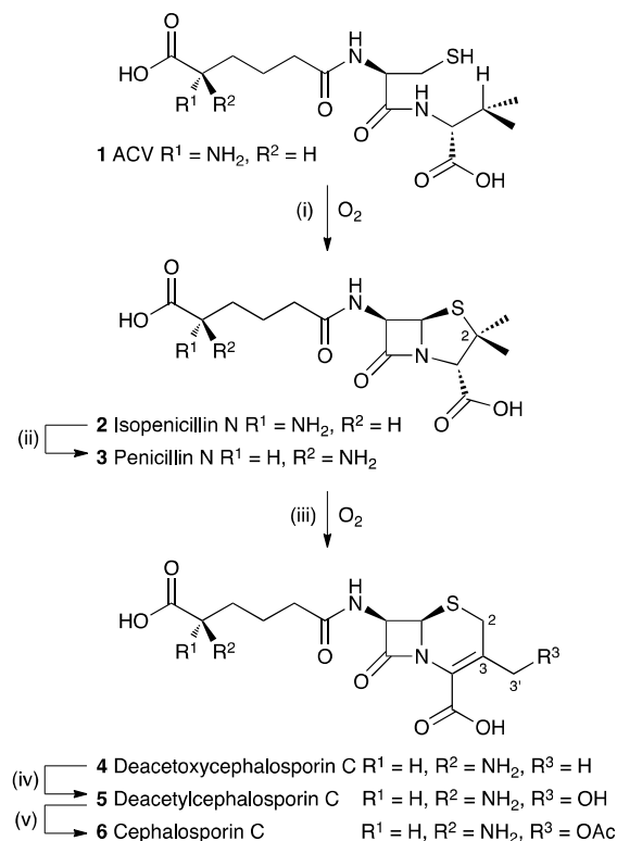
Scheme 1. Overall pathway from ACV 1 to cephalosporin C 6 . Enzymes: (i), Isopenicillin N synthase; (ii), Isopenicillin N epimerase; (iii) Deacetoxycephalosporin C synthase; (iv) Deacetylcephalosporin C Synthase; (v) Acetyl-coenzyme A:DAC O-acetyltransferase.
