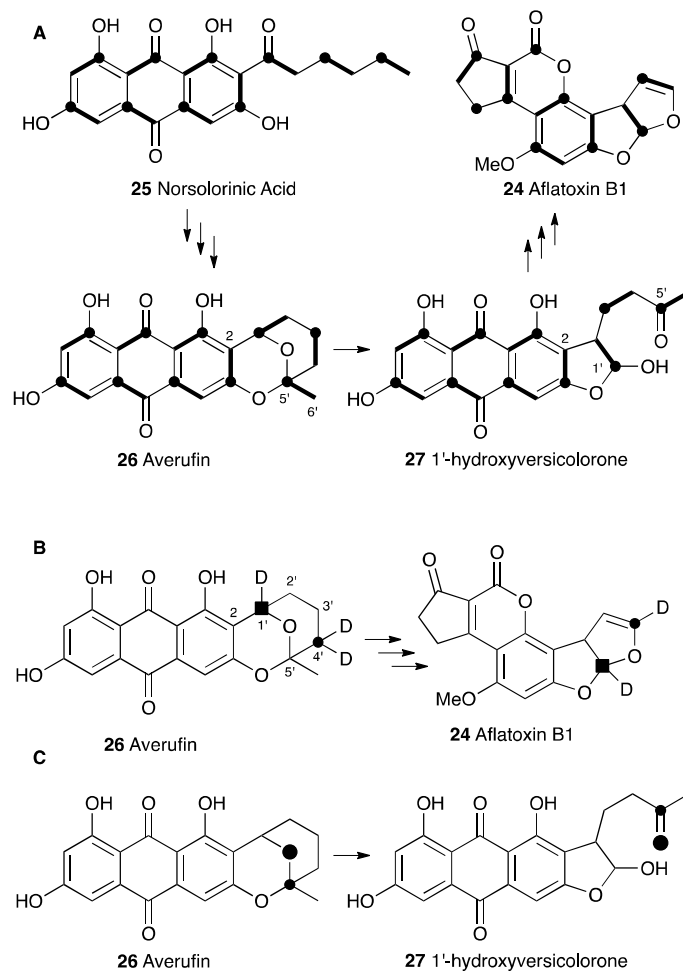
Scheme 7. A , Labelling patterns observed during the biosynthesis of aflatoxin B1. Bold bonds indicate intact acetate. Black circles indicate C-1 of acetate. B , selective labelling pattern during construction of the benzobisfuran system from averufin – results from 3 independent experiments shown together. C , retention of intact C-O bond observed via dual ^{13}\text{C} - ^{18}\text{O} labelling.
