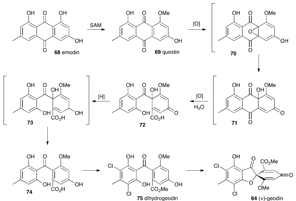
Scheme 13. Biosynthesis of geodin 64 in Aspergillus nidulans .
