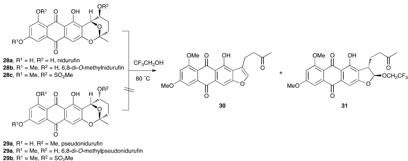
Scheme 8. Rearrangement of activated and protected 6,8-di-O-methylnidurufin epimers.
