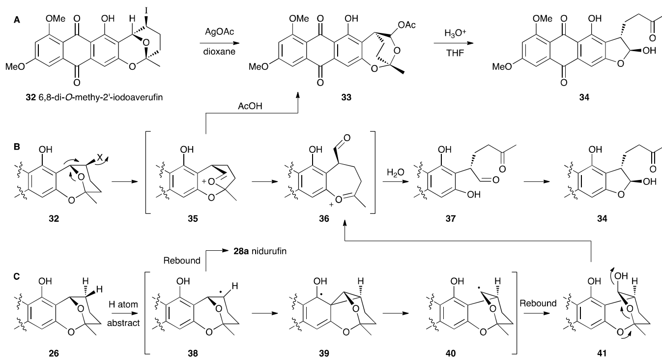
Scheme 9. A, In vitro reactions of 2'-iodoaverufin leading to the hydroxyversicolorone skeleton. B, Proposed mechanism accounting for the stereoselectivity of the rearrangement. C, Proposed reaction manifold stemming from cytochrome P450 catalysed hydrogen atom abstraction, followed by rearrangement and hydroxylation.
