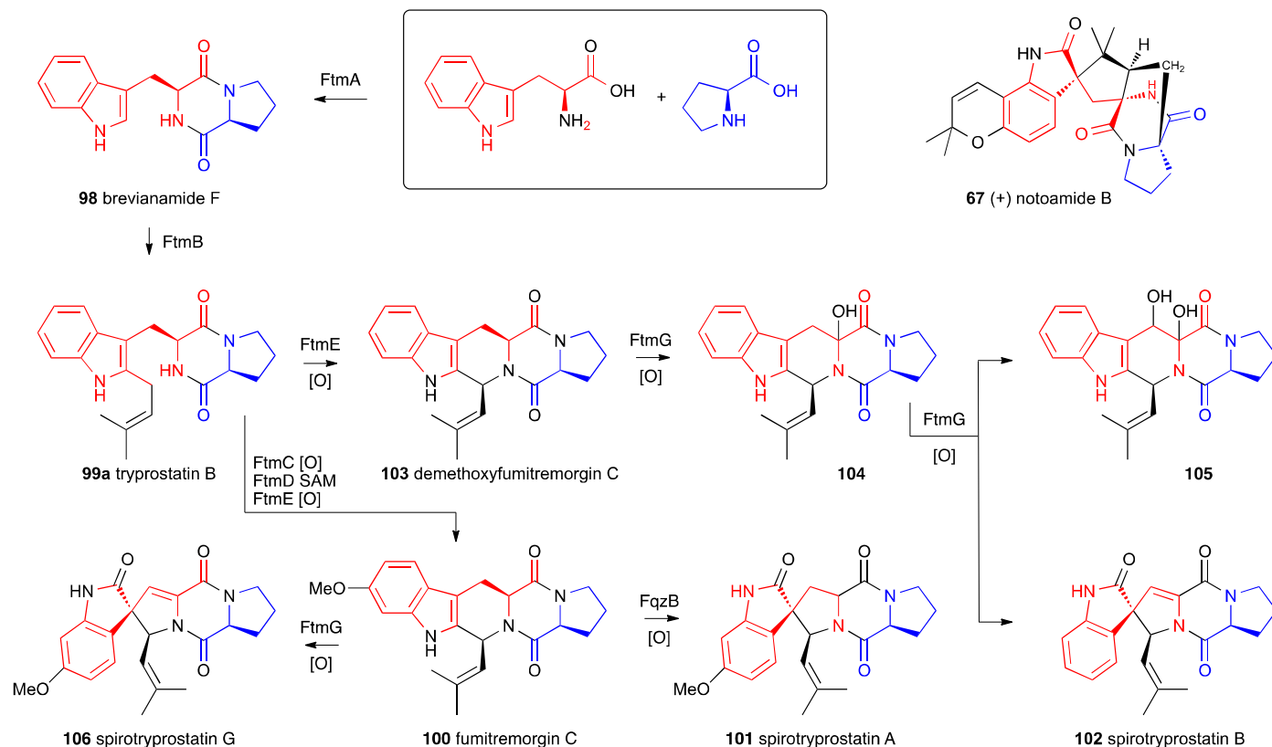
Scheme 17. Compounds derived from brevianamide F and the spirotryprostatin pathways.
