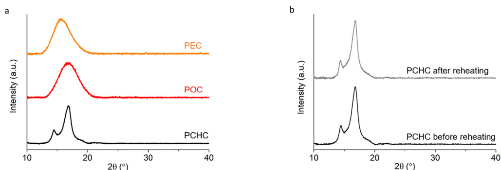
Fig. 4 WAXD spectra of (a) poly(ethylene camphorate) (PEC), poly(octamethylene camphorate) (POC) and poly(cyclohexanedimethylene camphorate) (PCHC), and (b) PCHC before and after reheating.
