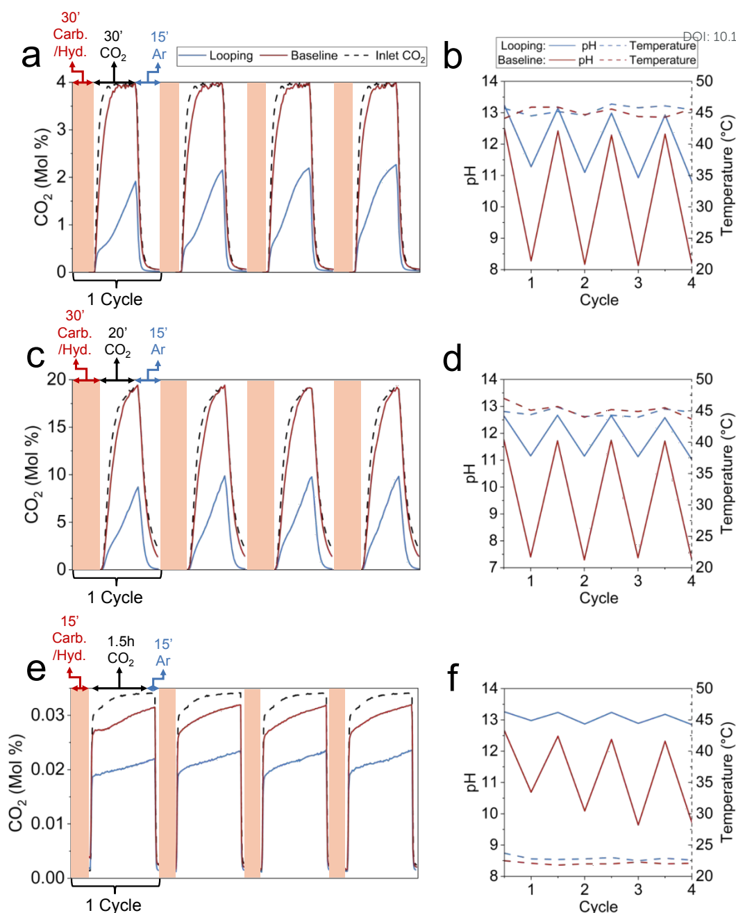
Fig. 2 (a) Four Na 2 CO 3 looping cycles of 4% CO 2 with quenched BOF slag compared to baseline; 1 g slag per cycle, 45°C, and 90 sccm 4% CO 2 /Ar. (b) pH and temperature after each step in 4% CO 2 looping and baseline. Half cycles are after carbonation and full cycles are after CO 2 capture. (c) Four Na 2 CO 3 looping cycles of 20% CO 2 with aged fines compared to baseline; 10 g slag per cycle, 45°C, and 90 sccm 20% CO 2 /Ar. (d) pH and temperature after each step in 20% CO 2 looping and baseline. (e) Four Na 2 CO 3 looping cycles of air CO 2 with quenched BOF slag compared to baseline; 0.05 g slag per cycle, 24°C, and 90 sccm 343 ppm CO 2 . (f) pH and temperature after each step in air CO 2 looping and baseline.
