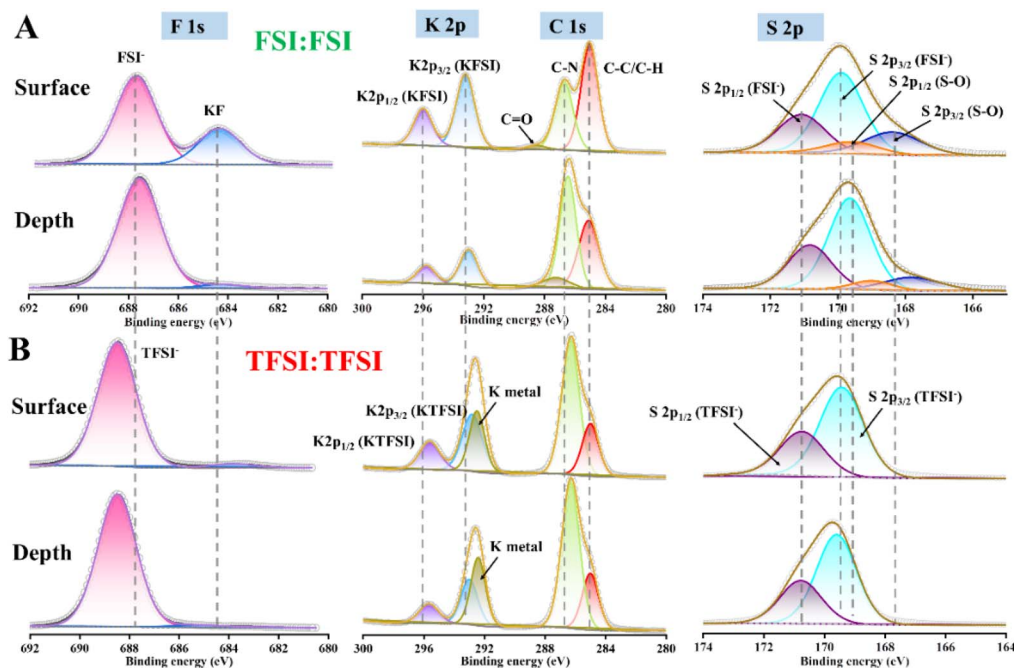
Fig. 6 XPS of the K metal surface and bulk (depth of 8 nm, Ar + etching speed of 0.8 nm min -1 ) after immersing for 28 days in (A) KFSI:Pyrr 12 O 1 FSI or (B) KFSI:Pyrr 12 O 1 TFSI solutions (the grey open points represent the experimental data, and the solid lines represent the fitting results).
