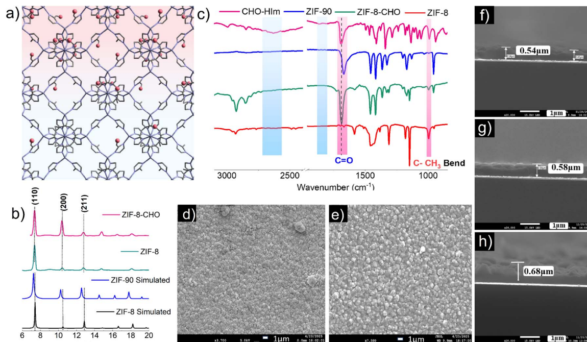
Fig. 1 (a) Illustration of the ZIF-8-CHO heterostructure thin film (red sphere = CHO group). (b) Out-of-plane XRD patterns of ZIF-8-CHO and ZIF-8 with simulated ZIF-8 and ZIF-90. (c) IRRAS of ZIF-8-CHO, ZIF-8, ZIF-90 (powder), and 2-imidazolecarboxaldehyde (powder). (d and e) SEM morphology of ZIF-8 and ZIF-8-CHO. (f–h) Cross-section SEM images of ZIF-8, ZIF-8-CHO, and ZIF-8-ZIF-90, respectively.
