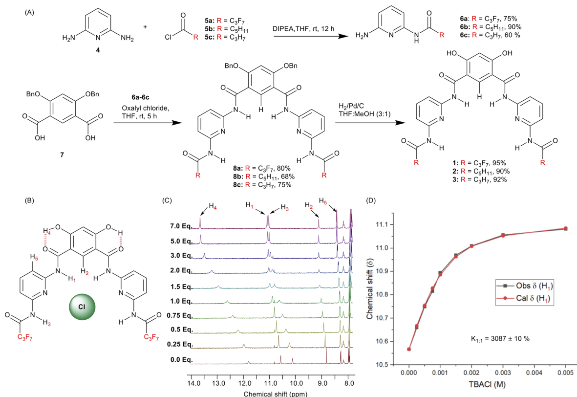
Fig. 2 (A) Synthesis of transporters 1–3. (B) Chemical structure of transporter 1 complexed to chloride. (C) 1 H NMR titration spectra for 1 (2.5 mM) in THF- d 8 with stepwise addition of TBACl in THF- d 8 . Protons assigned in panel B, and the equivalents of added TBACl are shown on the stacked spectra. (D) The plot of chemical shift (δ) of proton H 1 vs. concentration of TBACl added for transporter 1 , fitted to a 1 : 1 binding model using BindFit.
