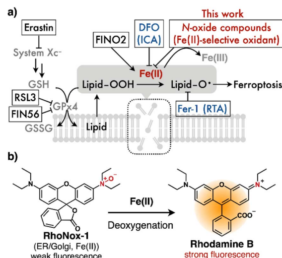
Fig. 1 (a) Schematic representation of the ferroptosis pathway. GSH: glutathione, GSSG: glutathione disulfide, GPx4: glutathione peroxidase 4, DFO (deferolamine, ICA: iron-chelating agents), and Fer-1 (ferrostatin-1, RTA: radical-trapping agents). Erastin and RSL-3 are ferroptosis inducers. (b) Structure and mechanism of RhoNox-1, a Fe(II)-selective fluorescent probe based on N -oxide chemistry.
