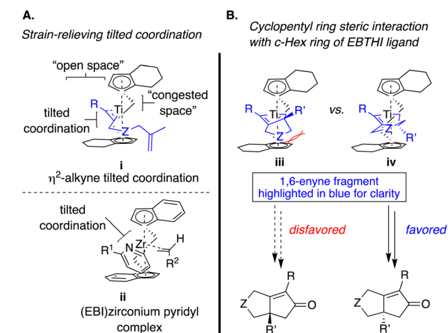
Scheme 7 Tilted coordination of alkyne or pyridyl ligand in the early-transition metal center (left); the proposed enantiodetermining transition state structures in the enantioselective Ti(II)-catalyzed PKR (right).
