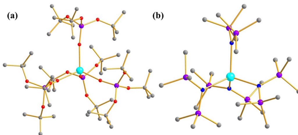
Fig. 11 The molecular structure of the complex (a) [\text{U}(\text{OSi}(\text{O}^t\text{Bu})_3)_4]^- ( 16 ) (b) [\text{U}(\text{N}(\text{SiMe}_3)_2)_4]^- ( 17 ). Colour code: U (cyan), O (red), N (blue), Si (violet), C (grey). Hydrogens and counter anions are omitted for clarity.
