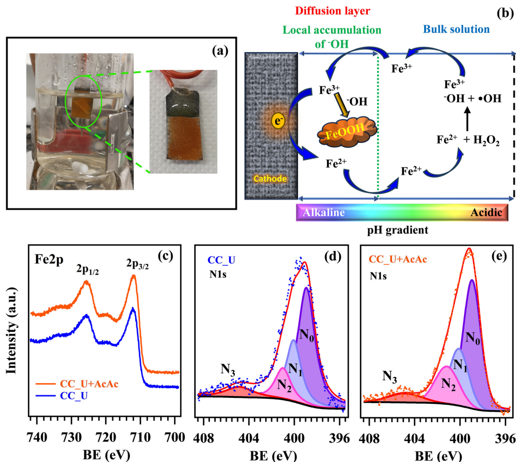
Fig. 8 (a) Image of the CC_U + AcAc sample after the test for 24 h as a working electrode in EF processes for FNT degradation. (b) Sketch of the route yielding insoluble \text{Fe(III)} deposits onto the electrode's surface. XPS signals after EF tests for \text{Fe}2p (c) and \text{N}1s (d and e).
