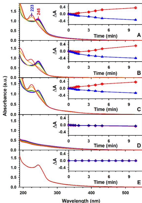
Fig. 1 UV-visible analysis during irradiation ( \lambda_{\text{cut-off}} \geq 295 nm) at pH 7.0 of (A) experiment with 30\ \mu\text{M} iohexol, 3.0\ \text{mg}\ \text{L}^{-1} humic acids, and 5.5\ \text{mg}\ \text{L}^{-1} \text{ClO}^- ; (B) control A in the absence of humic acids, (C) control B in the absence of \text{ClO}^- ; (D) control C in the absence of iohexol; and (E) control D in the absence of light. Monitored at irradiation time of (pink) 0, (purple) 0.25, (blue) 0.5, (green) 1, (yellow) 1.5, (orange) 5, and (red) 10 min. Insets display the mean absorbance change with time ( \Delta A_\lambda = A_t - A_0 ) for (red diamond) iodide at \lambda = 223 nm and (blue triangle) iohexol at \lambda = 245 nm. Error bars are represented but are smaller than the symbols.
