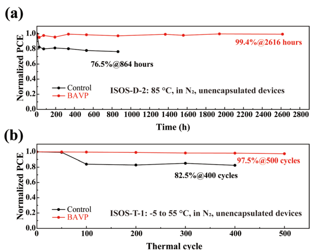
Fig. 5 (a) Thermal stability test of the unencapsulated PSCs at 85 \text{ }^\circ\text{C} in \text{N}_2 following the ISOS-D-2 protocol. (b) Thermal-cycling stability test of the unencapsulated PSCs at a temperature range of -5 to 55 \text{ }^\circ\text{C} in \text{N}_2 following the ISOS-T-1 protocol.
