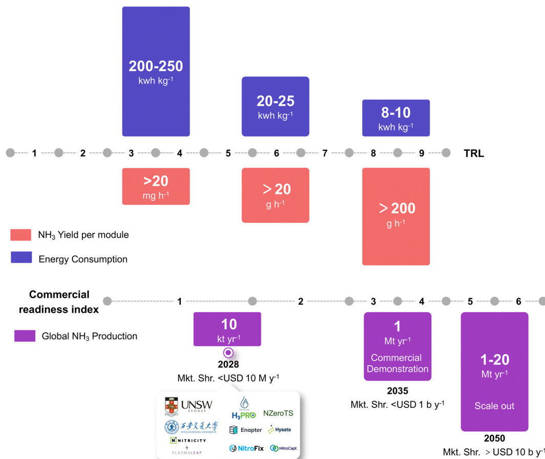
Fig. 16 Commercialisation roadmap for NORR, illustrating TRL milestones, module-level performance benchmarks, alignment with commercial readiness levels, and projected contribution to the global ammonia market by 2050.
