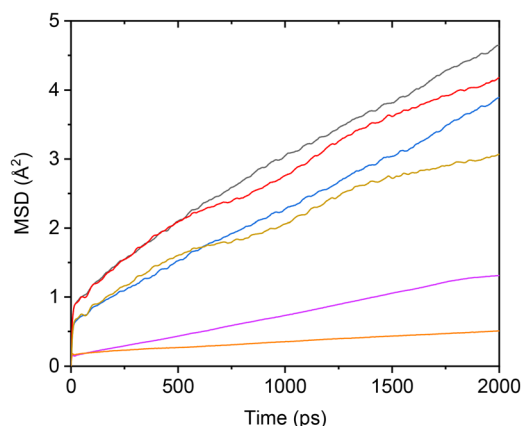
Fig. 5 MSDs simulated for \text{TiO}_2 -filled PEC/LiTFSI SCE models under different conditions. Data are shown for \text{Li}^+ at salt concentrations of 40 mol% (black) and 120 mol% (red), TFSI(bulk) at salt concentrations of 40 mol% (blue) and 120 mol% (dark yellow), and TFSI(interface) at salt concentrations of 40 mol% (purple) and 120 mol% (orange).
