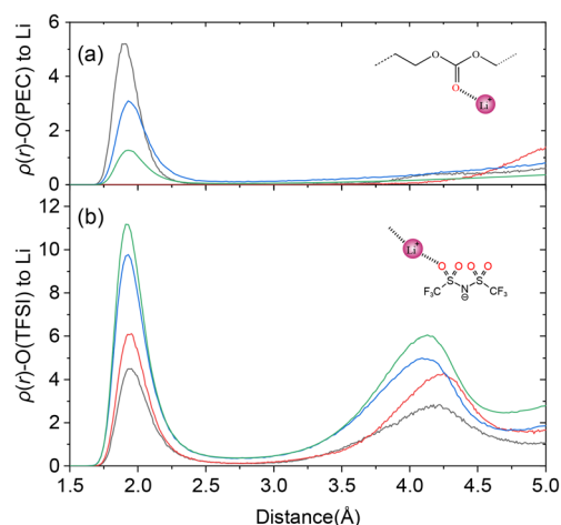
Fig. 3 RDFs simulated for PEC/LiTFSI SCE and \text{TiO}_2 -filled SCE models between Li cations and oxygen atoms from (a) carbonyl groups in polymer chains and (b) TFSI anions. RDF curves are coloured based on salt concentration: 40 mol% SCE (black), 120 mol% SCE (red), 40 mol% SPE (blue) and 120 mol% SPE (green).
