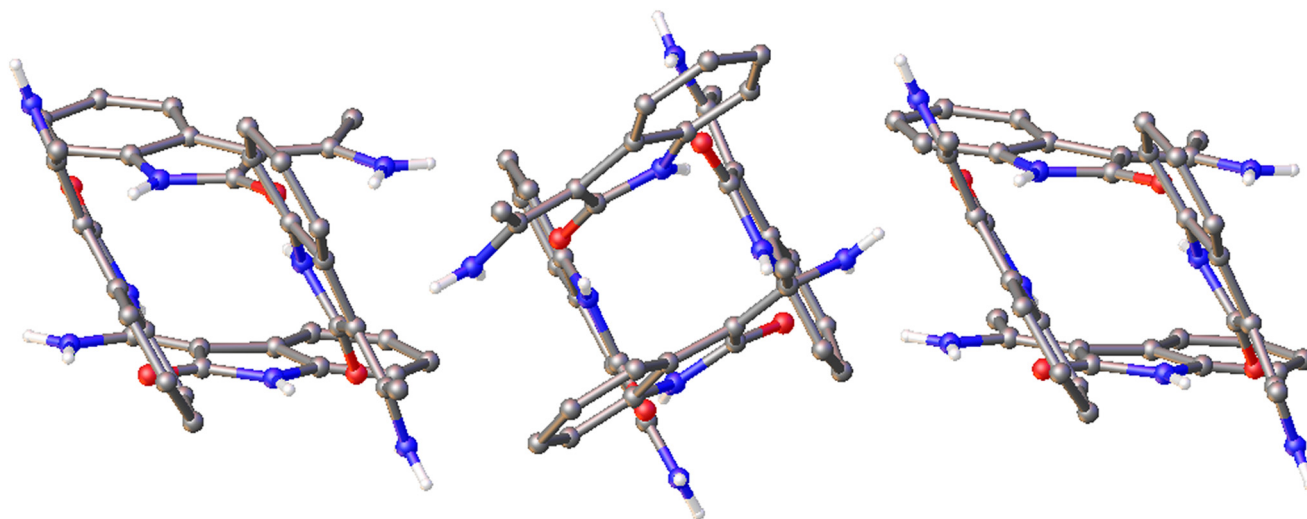
Fig. 8 The asymmetric unit of IQEQT viewed down the crystallographic [100] directions.
