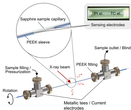
Fig. 1 Sample environment for combined in situ electrical impedance and X-ray characterization.
