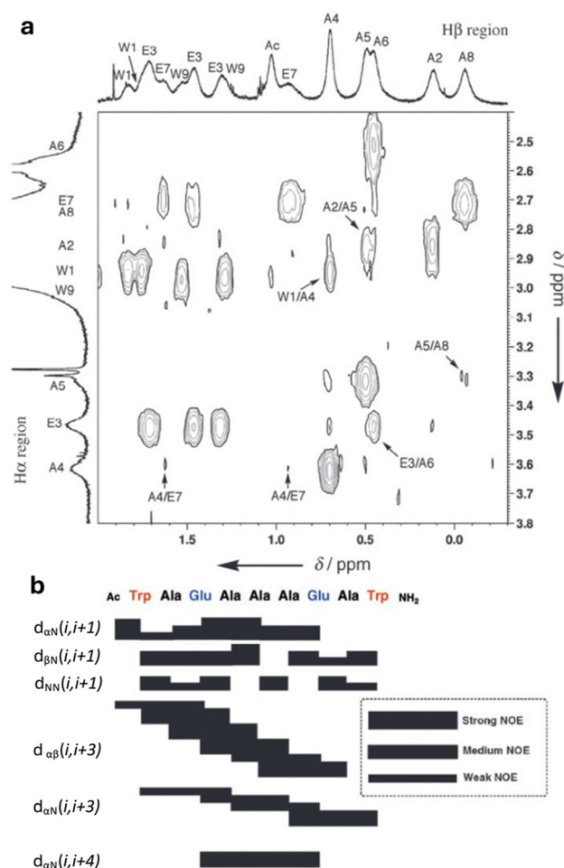
Figure 3 (a) Selected NOESY spectrum for the assignment of bound peptide (600 MHz, H 2 O/D 2 O = 9/1, 27 °C, 100 mM phosphate buffer, pH 6.8), [2] = 10 mM, [peptide] = 2.5 mM. Proton resonances labelled with single letter amino acid code and residue number corresponding to peptide in Fig. 2a; (b) NOE correlations for peptide 2 . Reproduced with permission from ref. 16.
