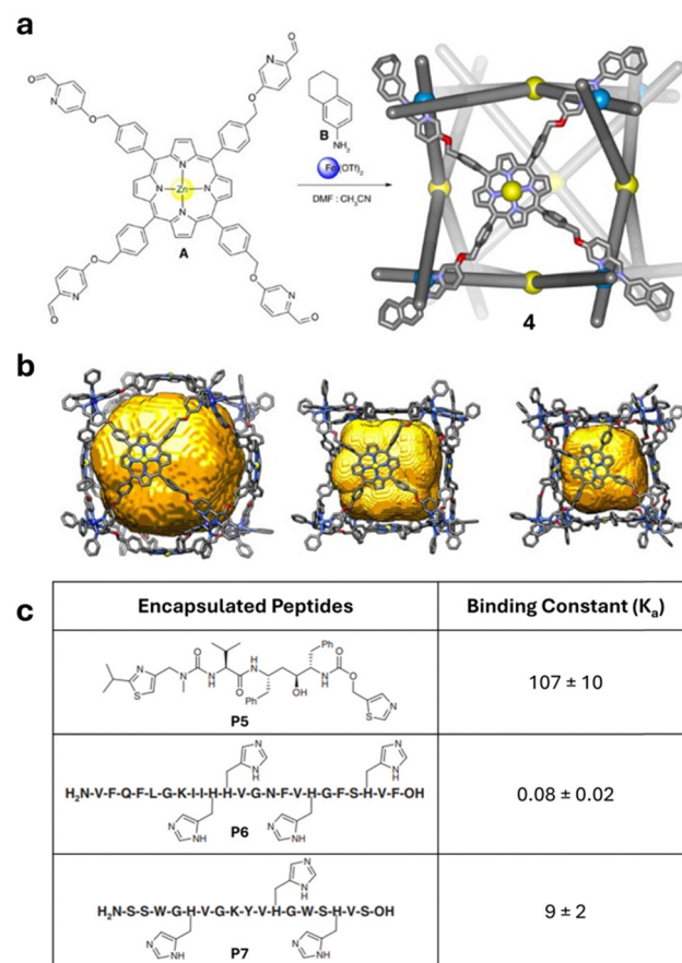
Figure 4 (a) Self-assembly of 4 , a cubic MOC with one zinc porphyrin per face; (b) MM2 energy minimised models of 4 showing the structural flexibility and variable void volumes from 10 083 to 3143 Å 3 ; (c) peptides P5–P7 found to bind within 4 and their binding constants. Reproduced with permission from ref. 6.
