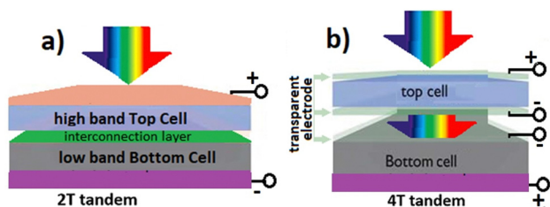
Fig. 14 Schematic example of (a) 2T tandem and (b) 4T tandem.
