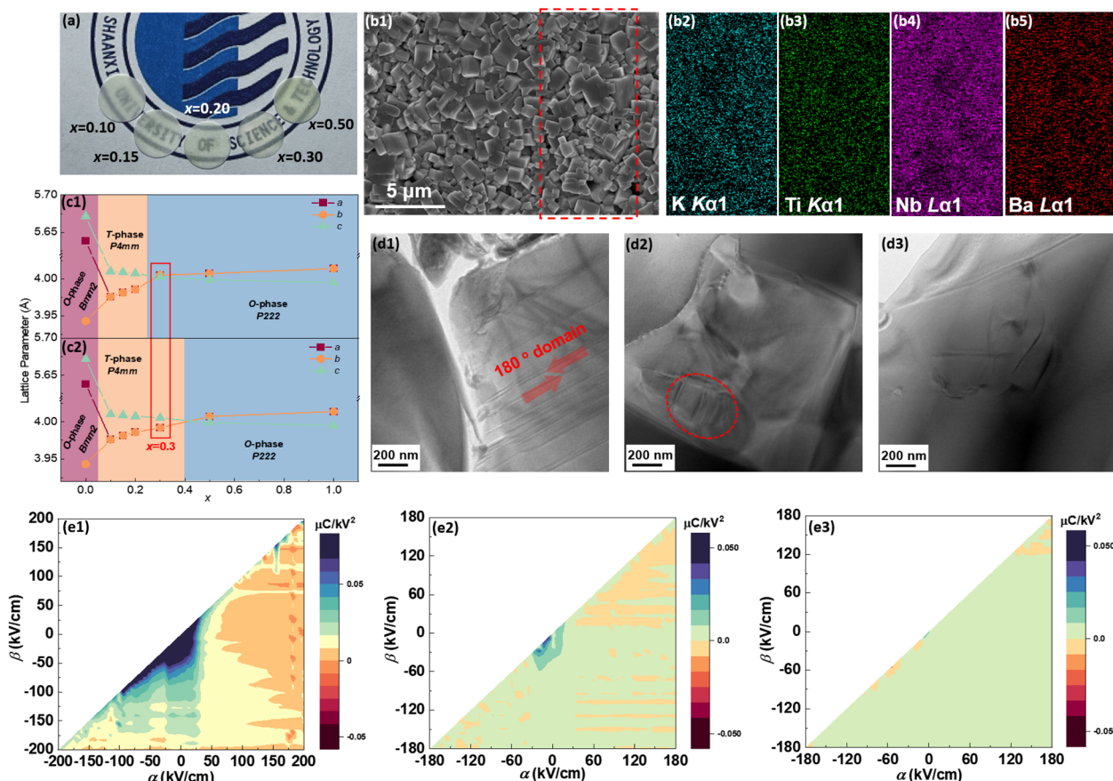
Fig. 1 (a) Picture of (1 - x)\text{KNN}-x\text{BCZT} ceramics with different x ; (b1) SEM image of 0.7KNN–0.3BCZT; (b2)–(b5) EDS mappings for K, Ti, Nb, and Ba of the area circled by the red dashed rectangle in (b1); (c1) and (c2) the variation between the lattice parameter and x ; (d1)–(d3) TEM images of (1 - x)\text{KNN}-x\text{BCZT} ceramics with x = 0.1, 0.3 , and 0.5 ; (e1)–(e3) the FORC distribution of (1 - x)\text{KNN}-x\text{BCZT} ceramics with x = 0.1, 0.3 , and 0.5 .
