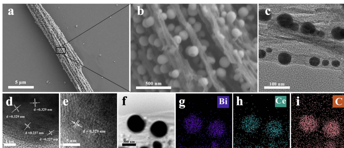
Fig. 1 Microstructure characterization of \text{Ce}_2\text{-Bi@C} . (a) SEM image. (b) Localized magnified image of (a). (c) TEM image. (d and e) HRTEM images. (f–i) EDS mappings.
