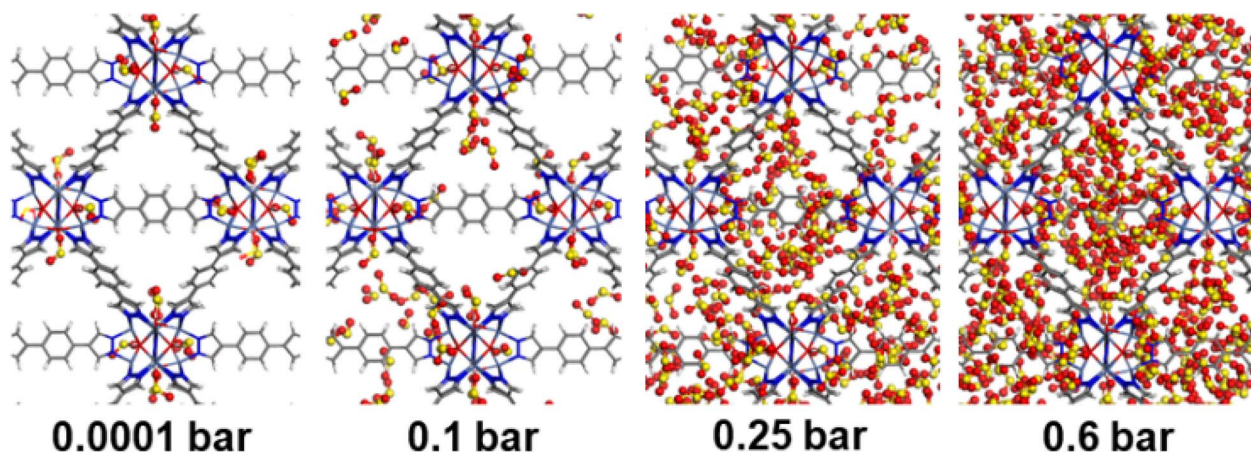
Fig. 5 GCMC simulated adsorption sequence of \text{SO}_2 in \text{NiBDP-0H}_2\text{O} at 298 K, and at different pressures. \text{SO}_2 atom color codes: red (O), yellow (S). MOF atom color codes: red (O), gray (C), blue (N), white (H), purple (Ni).
