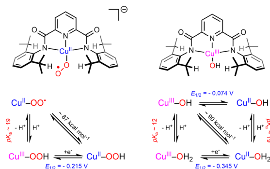
Scheme 6 Comparison of the thermodynamic properties of [(L)\text{Cu}^{\text{II}}(\eta^1\text{-O}_2)]^- and [(L)\text{Cu}^{\text{III}}(\text{OH})] using the same bis(arylcarboxamido)-pyridine ligand. Adapted from ref. 103.
