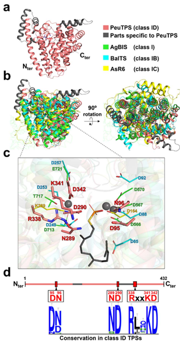
Fig. 4 Structure of PeuTTPS. (a) 3D structure of PeuTTPS predicted by AlphaFold2. (b) Superposition of the 3D structure of PeuTTPS (pink and gray) with the class I TPS domain of AgBIS (green), BalTS (class IB; blue), and AsR6 (class IC; yellow). The model of PeuTTPS has a sufficient confidence level in the region superposed with other TPSs (Fig. S1†). Additionally, the RMSD of PeuTTPS and class I TPS domain of AgBIS (3.1) is comparable to that of the crystal structures, AgBIS-BalTS and AgBIS-AsR6 (both 3.7). (c) Proposed catalytic residues of PeuTTPS (pink) superposed with that of AgBIS (green), BalTS (blue), and AsR6 (yellow). A side chain of farnesyl thiopyrophosphate and Mg^{2+} ion co-crystallized with AgBIS are represented as gray sticks and gray spheres, respectively. (d) Conservation of proposed catalytic residues in class ID TPSs. The height of the symbols in the sequence logos indicates the sequence conservation in 120 homologs at that position.
