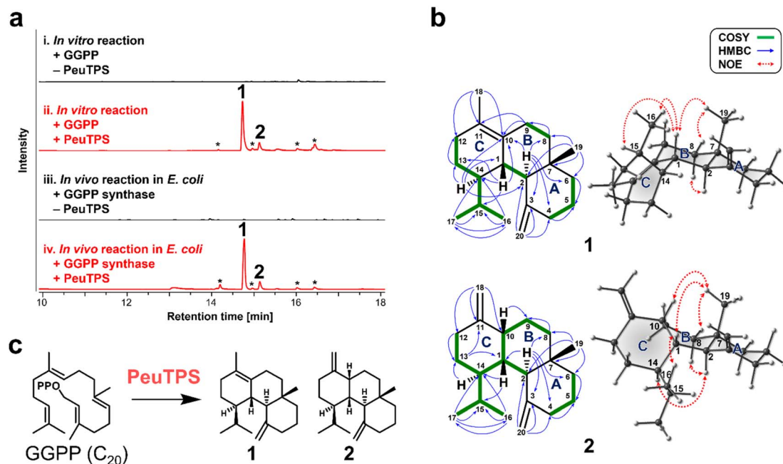
Fig. 3 Analysis of PeuTPS products. (a) Gas chromatography–mass spectrometry analyses (total ion chromatograms) of PeuTPS products from GGPP by in vitro and in vivo reactions. (i) and (ii) Reaction products formed from GGPP in the absence (i) and presence (ii) of PeuTPS. (iii) and (iv) Metabolites of E. coli that expressed (iv) and did not express (iii) PeuTPS with GGPP synthase and mevalonate pathway enzymes. Asterisks indicate unidentified products. (b) Chemical structures of 1 and 2 . The most stable 3D structures obtained by the conformational search are presented on the right. Characteristic 2D NMR correlations are shown. (c) Reaction catalyzed by PeuTPS.
