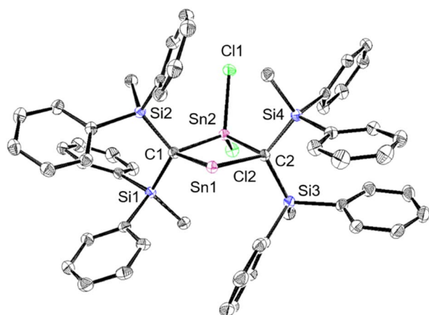
Fig. 6 Molecular structure of 5Cl in the crystalline state with thermal ellipsoids at 50% probability; hydrogen atoms are omitted for clarity. Selected bond lengths [Å] and angles [°] for 5Cl : \text{Sn}1 \cdots \text{Sn}2 : 3.1022(5), \text{C}1\text{--}\text{Sn}1 : 2.313(2), \text{C}2\text{--}\text{Sn}1 : 2.301(2), \text{C}1\text{--}\text{Sn}2 : 2.163(2), \text{C}2\text{--}\text{Sn}2 : 2.173(2), \text{C}1\text{--}\text{Si}1 : 1.905(2), \text{C}1\text{--}\text{Si}2 : 1.888(2), \text{C}2\text{--}\text{Si}3 : 1.902(2), \text{C}2\text{--}\text{Si}4 : 1.909(2), \text{C}1\text{--}\text{Sn}1\text{--}\text{C}2 : 87.93(8), \text{C}1\text{--}\text{Sn}2\text{--}\text{C}2 : 95.22(8), \text{Sn}1\text{--}\text{C}1\text{--}\text{Sn}2 : 87.67(8), and \text{Sn}1\text{--}\text{C}2\text{--}\text{Sn}2 : 78.76(8).
