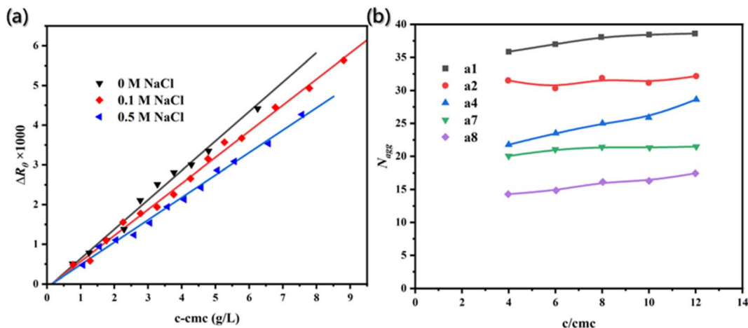
Fig. 4 (a) Excess scattering ratios ( \Delta R_{\theta} ) is the function of micellar concentration. 89 Reproduced with permission from ref. 89. Copyright 2007, Elsevier. (b) Aggregation number ( N_{agg} ) as a function of concentration c/cmc with different carbon atomic number ( s ) spacing between two dodecyl chains and a diamide spacer. 90 Reproduced with permission from ref. 90. Copyright 1999, American Chemical Society.
