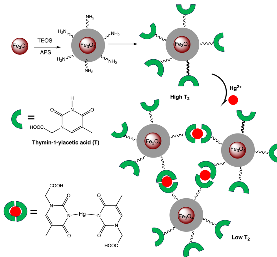
Scheme 17 Graphic for \text{Fe}_3\text{O}_4@SiO_2 -T NPs preparation and \text{Hg}(\text{II}) detection mechanism.
