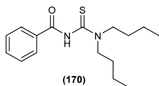
Fig. 95 Structure of N -benzoyl- N',N' -dibutyl thiourea.
