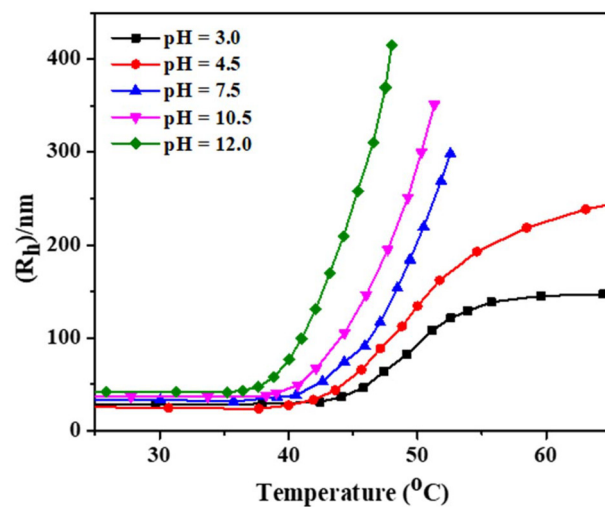
Fig. 8 Variations in hydrodynamic radius ( R_h ) of HNC-18 in an aqueous solution with temperature and pH.
