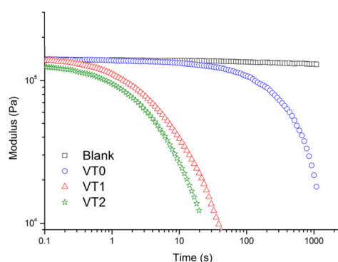
Fig. 5 Stress relaxation analysis of control crosslinked network "blank", vitrimer VT0, VT1 and VT2 at 160\text{ }^\circ\text{C} as function of time.
